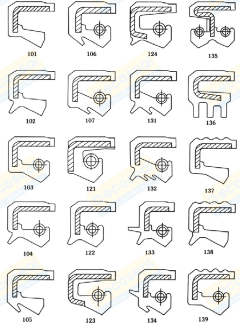
Charts of sog designs for oil seals Designs of rubber outer diameter
